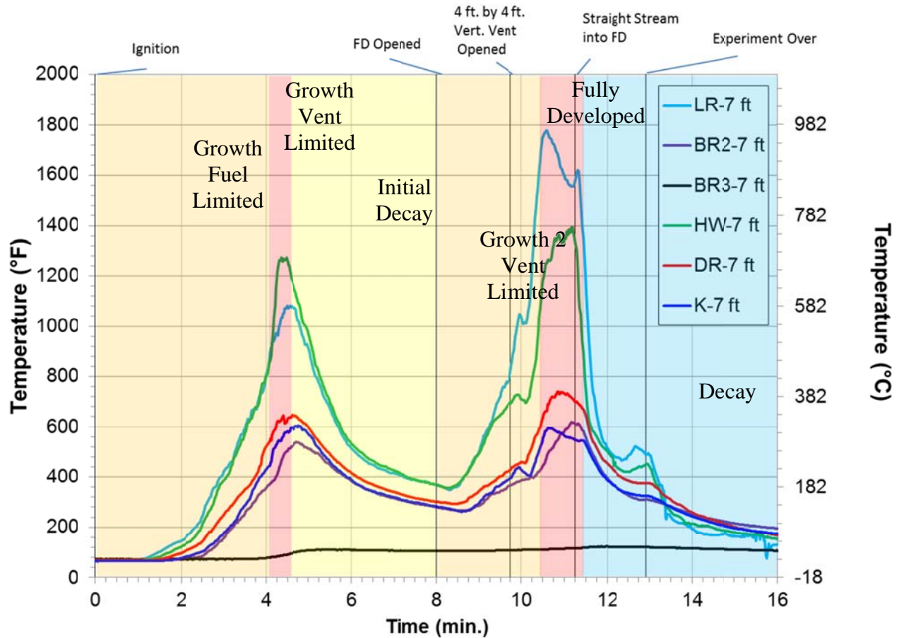
Figure 4.13: Experiment 5 Stages of Fire Development
