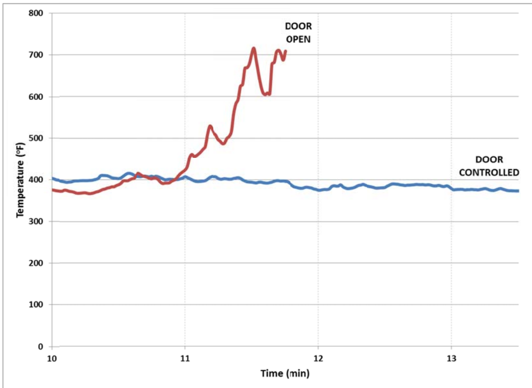
Figure 4.4: Two-Story Family Room Temperatures after Front Door Open and Before Roof Open
