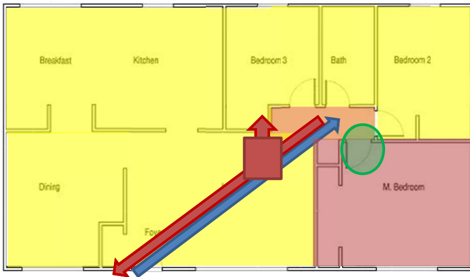
Figure 4.15: Flow path through another room to the seat of the fire
