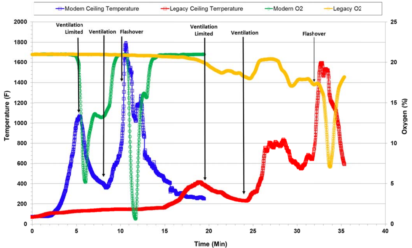
Figure 4.1: Modern vs. Legacy Temperatures and Oxygen Concentration Comparison
