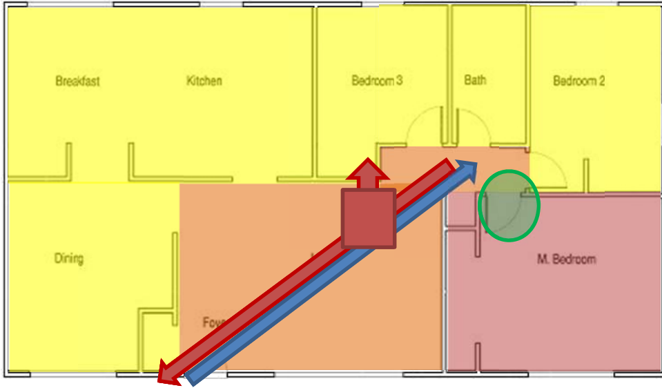
Figure 4.16: Flow path as furnishings are ignited in the living room
