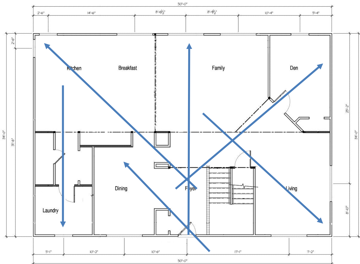
Figure 4.42: 2-story open floor plan with hose stream reaches
