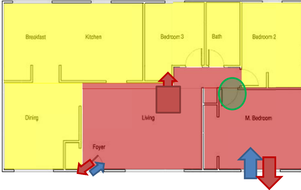
Figure 4.18: Flow paths after front bedroom window is opened
