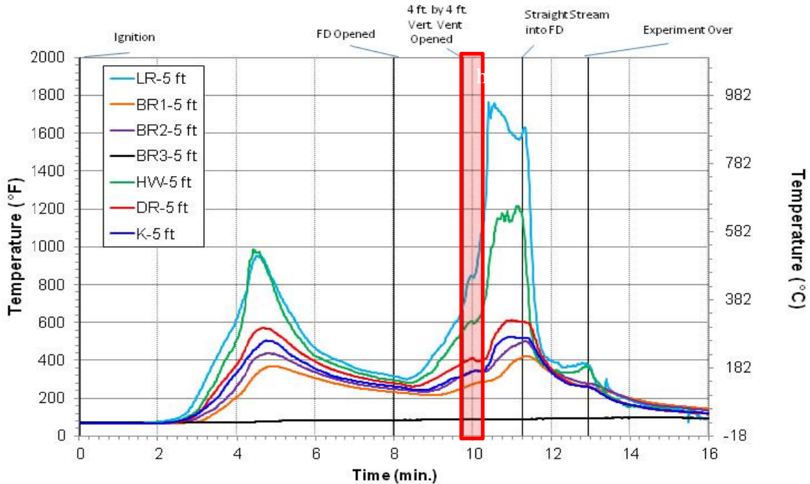
Figure 4.7: 5 ft. temperatures in the one-story house showing coordination window
