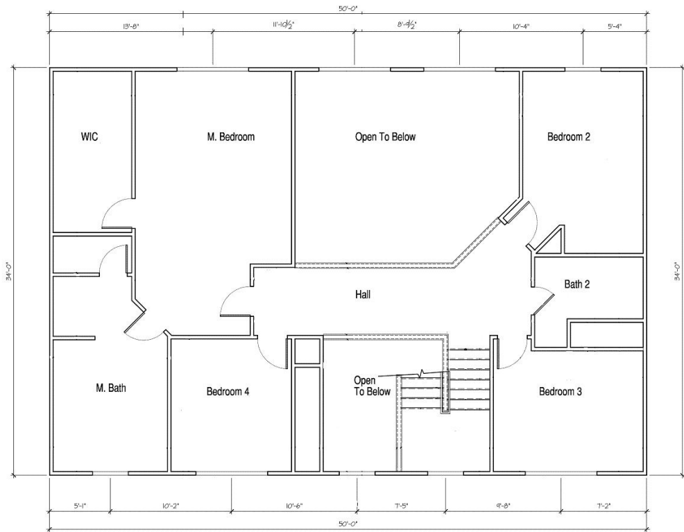
Figure 3.12. Two-Story House Second Floor Plan
