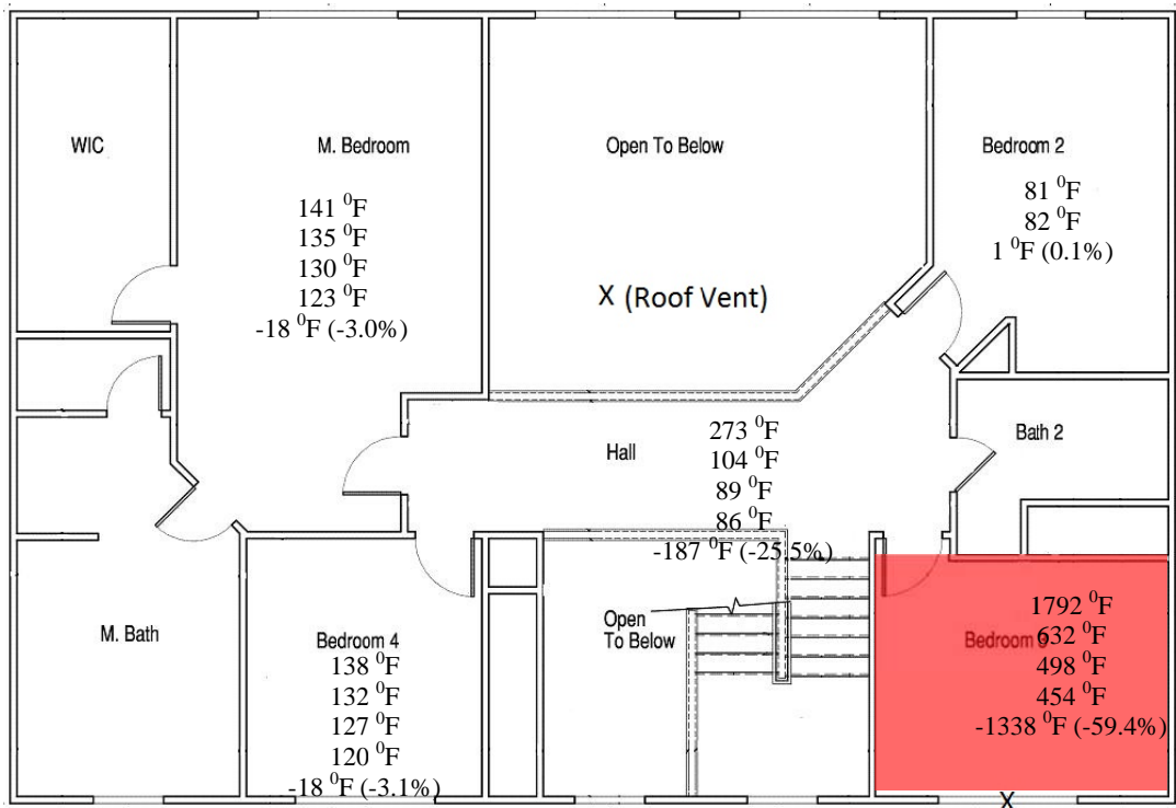
Figure 4.29: Experiment 14, Second Floor, Straight Stream
