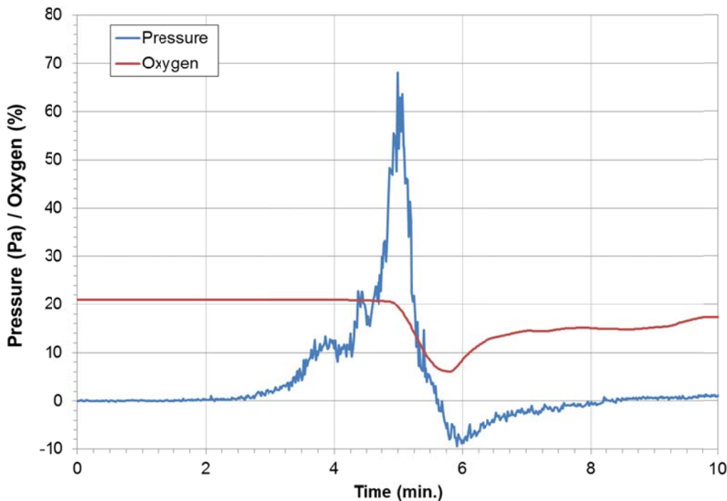
Figure 4.22: Pressure and Oxygen Concentrations that Impact Smoke Showing
