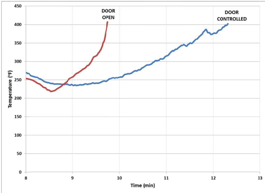
Figure 4.3: One-Story Living Room Temperatures after Front Door Open and Before Roof Open
