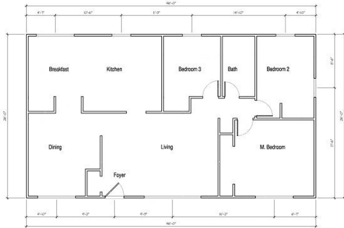
Figure 3.4: One-Story House Floor Plan
