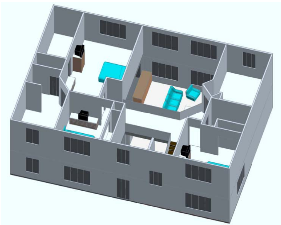
Figure 3.9. 3D Rendering of the 2-Story House from the Front
