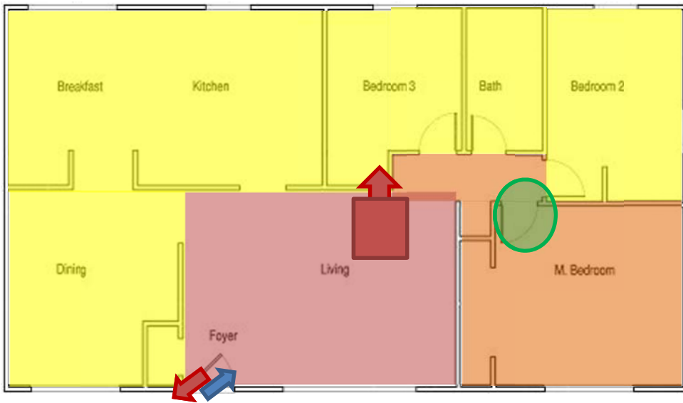
Figure 4.17: Flow path after the living room reaches flashover
