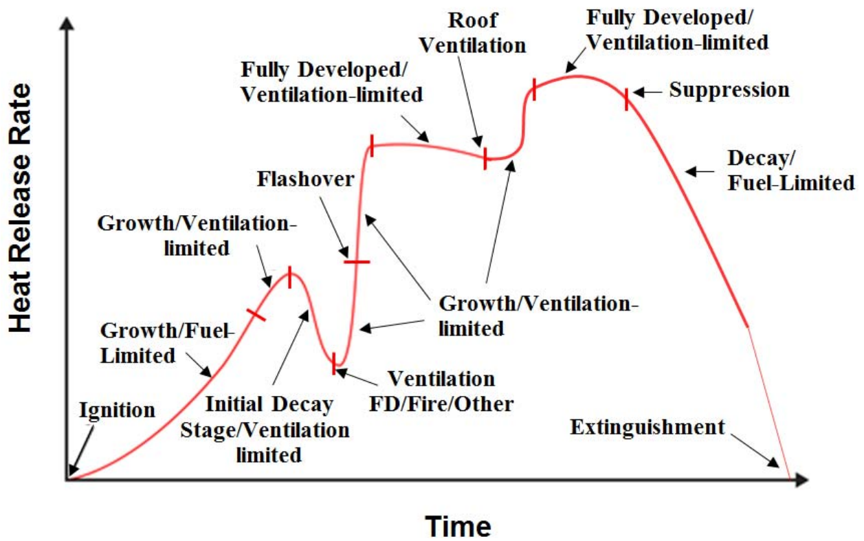
Figure 4.12: Fire growth curve for this fire example
